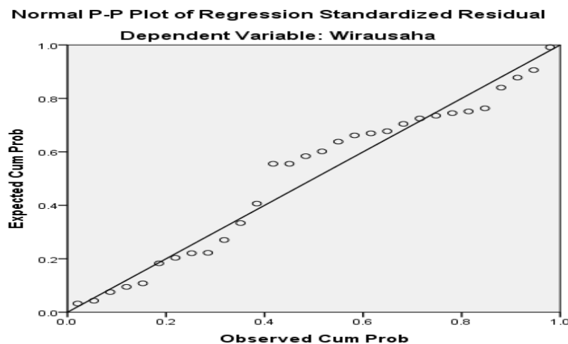
Gambar 4.1 :Grafik Hasil Pengujian Normal Probability Plot
