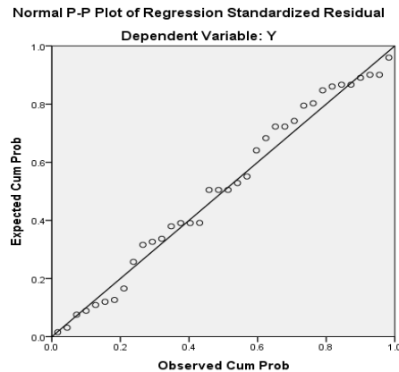
Grafik Probability-Plot
