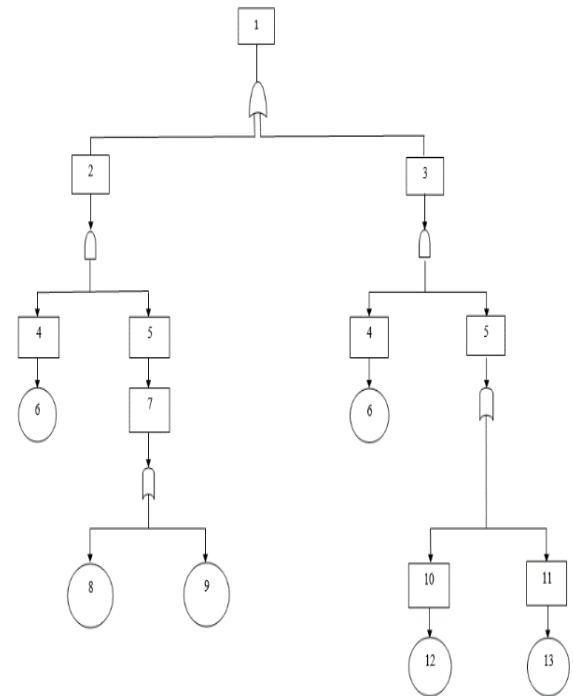
Gambar 5. Bagan Cut Set Fault Tree
