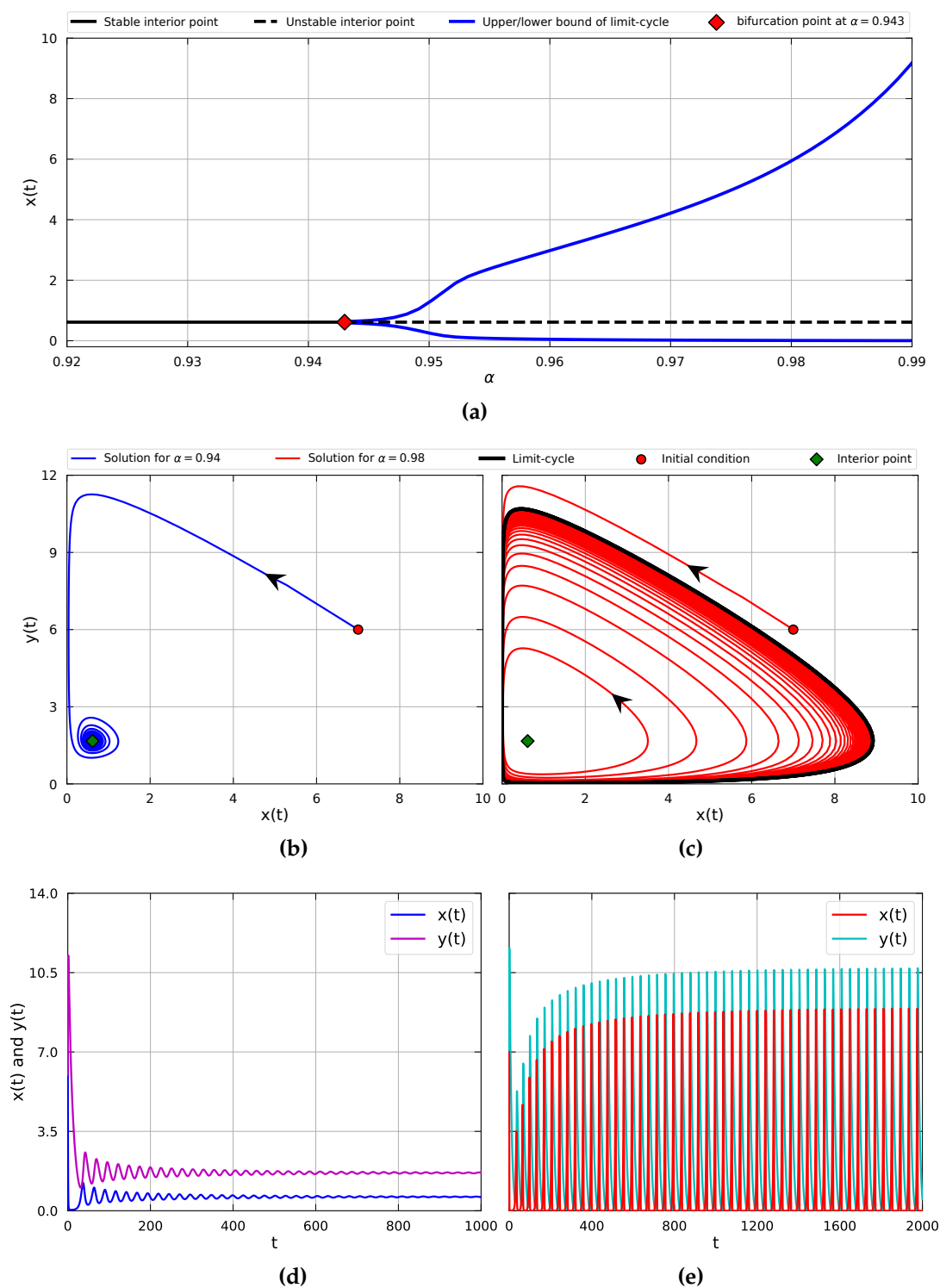
Figure 1. Numerical simulations of model (3) with parameter values: a = 0.5 , b = 0.3 , c = 0.25 , d = 0.1 , m = 0.1 , and n = 0.2 (a) Bifurcation diagram driven by \alpha in interval [0.92, 0.99] (b) Phase portrait when \alpha = 0.94 (c) Phase portrait when \alpha = 0.98 (d) Time series when \alpha = 0.94 (e) Time series when \alpha = 0.98
