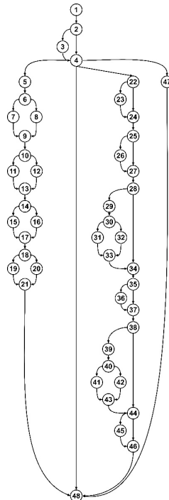
Gambar 10. Flow Graph Pengujian Whitebox Pada Proses Input, Edit, Delete Permohonan Akta Kematian
