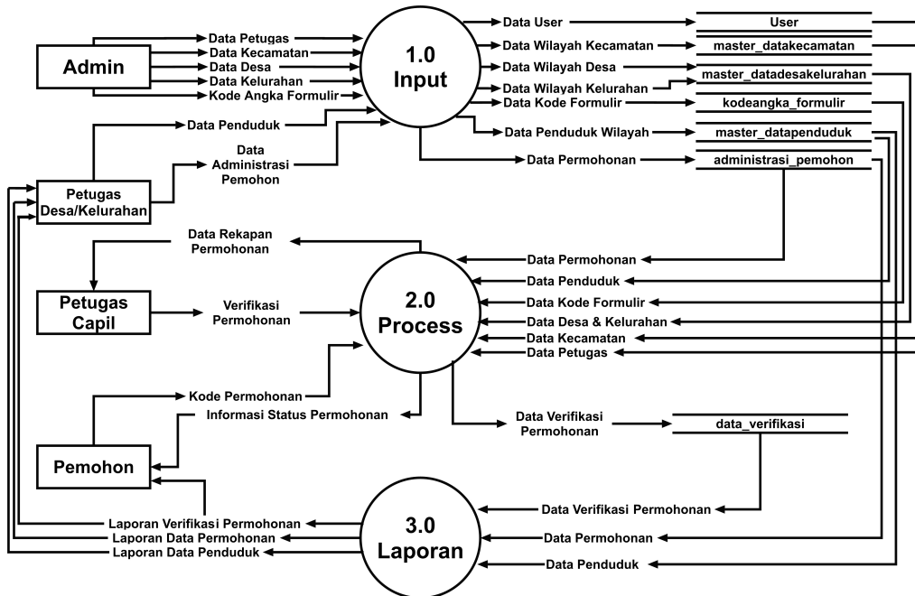
Gambar 3. Diagram Alir Data
