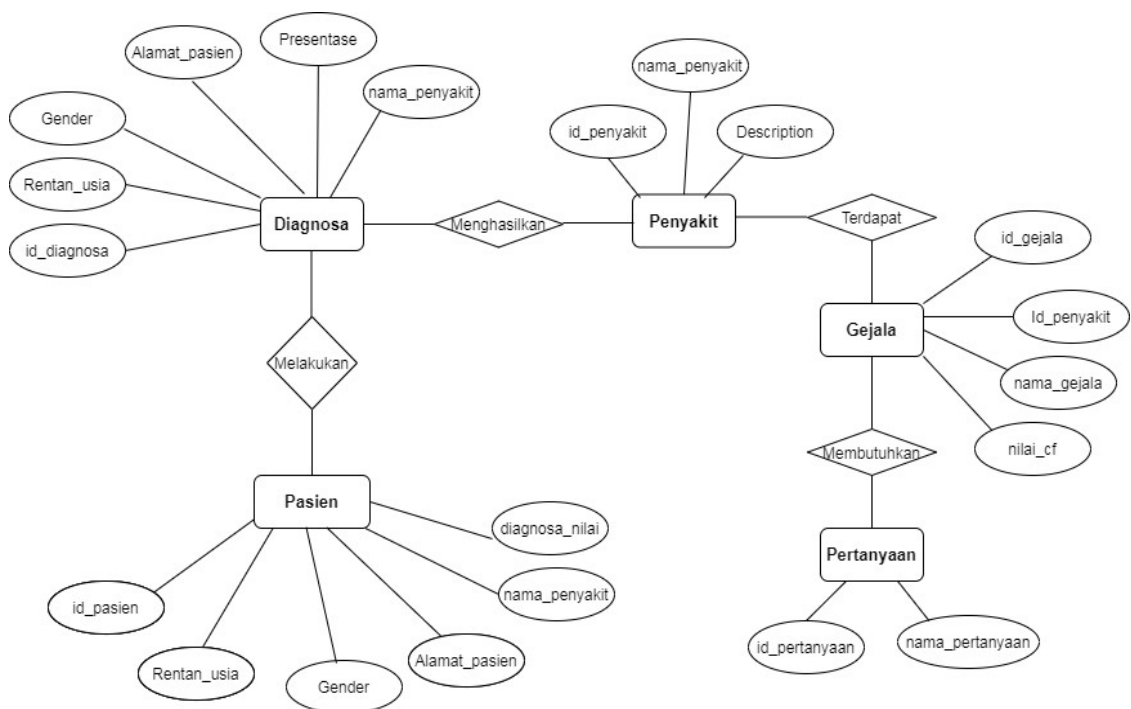
Gambar 4. ERD System
