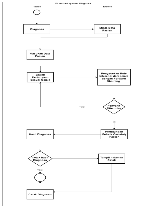
Gambar 5. Flowchart Diagnosa
