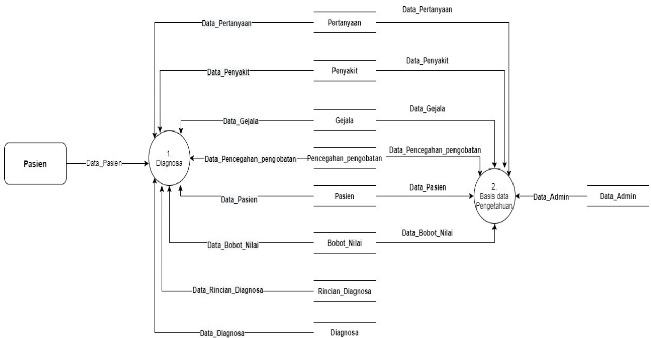
Gambar 3. DFD Level 1
