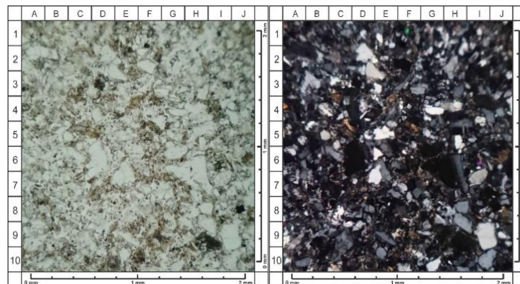
Gambar 9. Sayatan tipis batupasir
