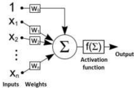
Gambar 3. Model Neural Network [12]
