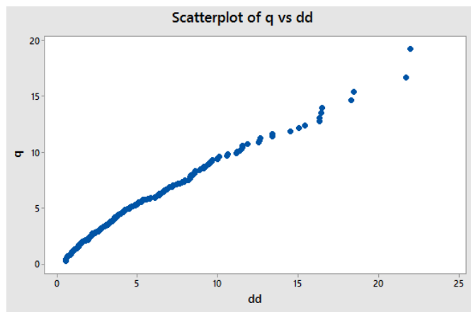
Gambar 1. Plot distribusi normal multivariat
